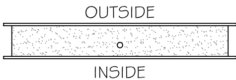
TYPE 6: BLOCK SPLINE I-JOIST SPLINE 2x LUMBER SPLINE
